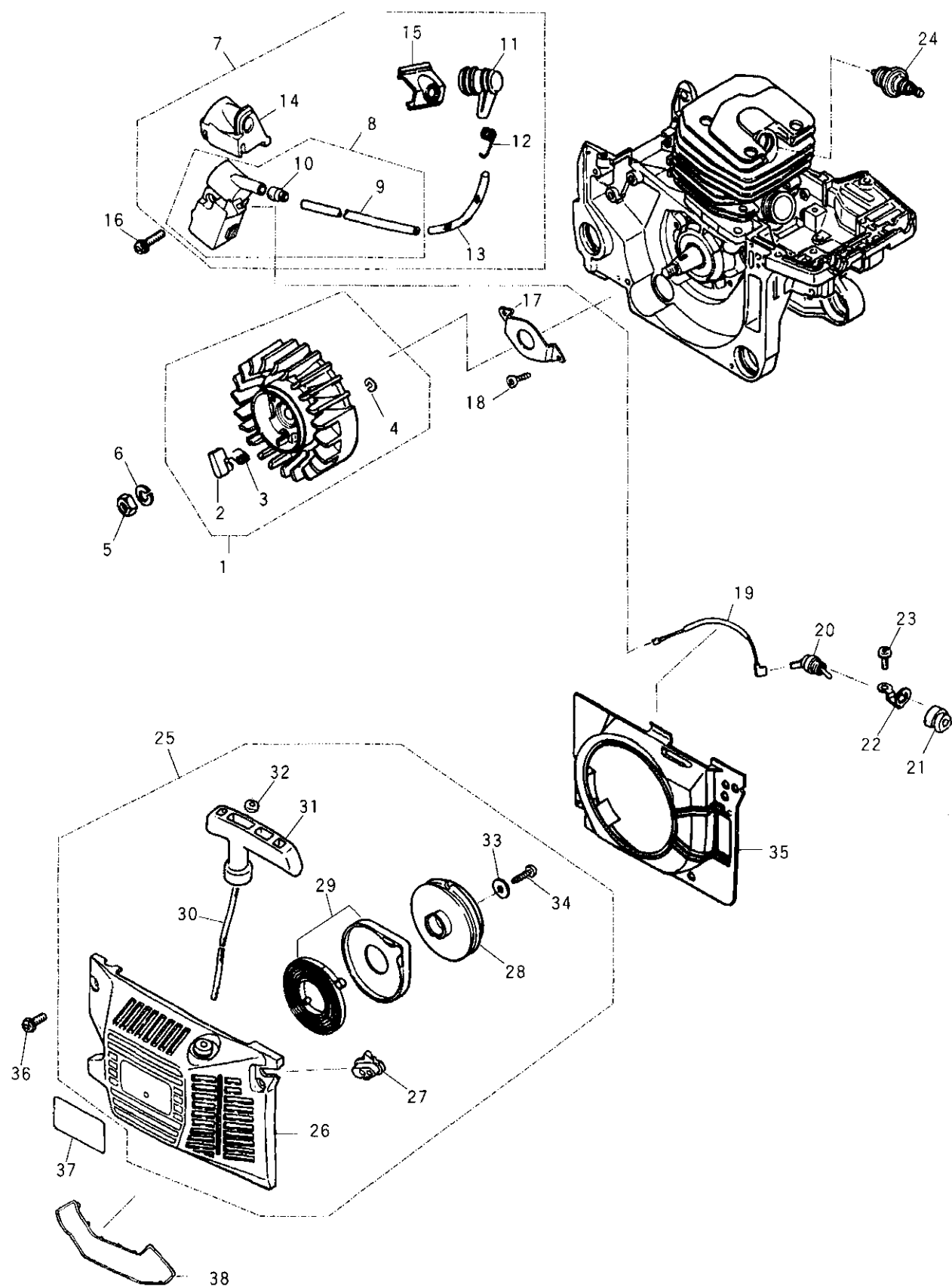
Fig. 2 IGNITION SYSTEM, STARTER
