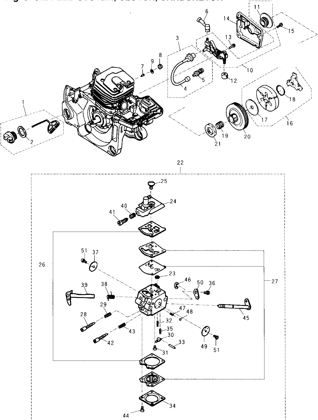
Fig. 5 OIL FEED SYSTEM, CLUTCH, CARBURETOR
