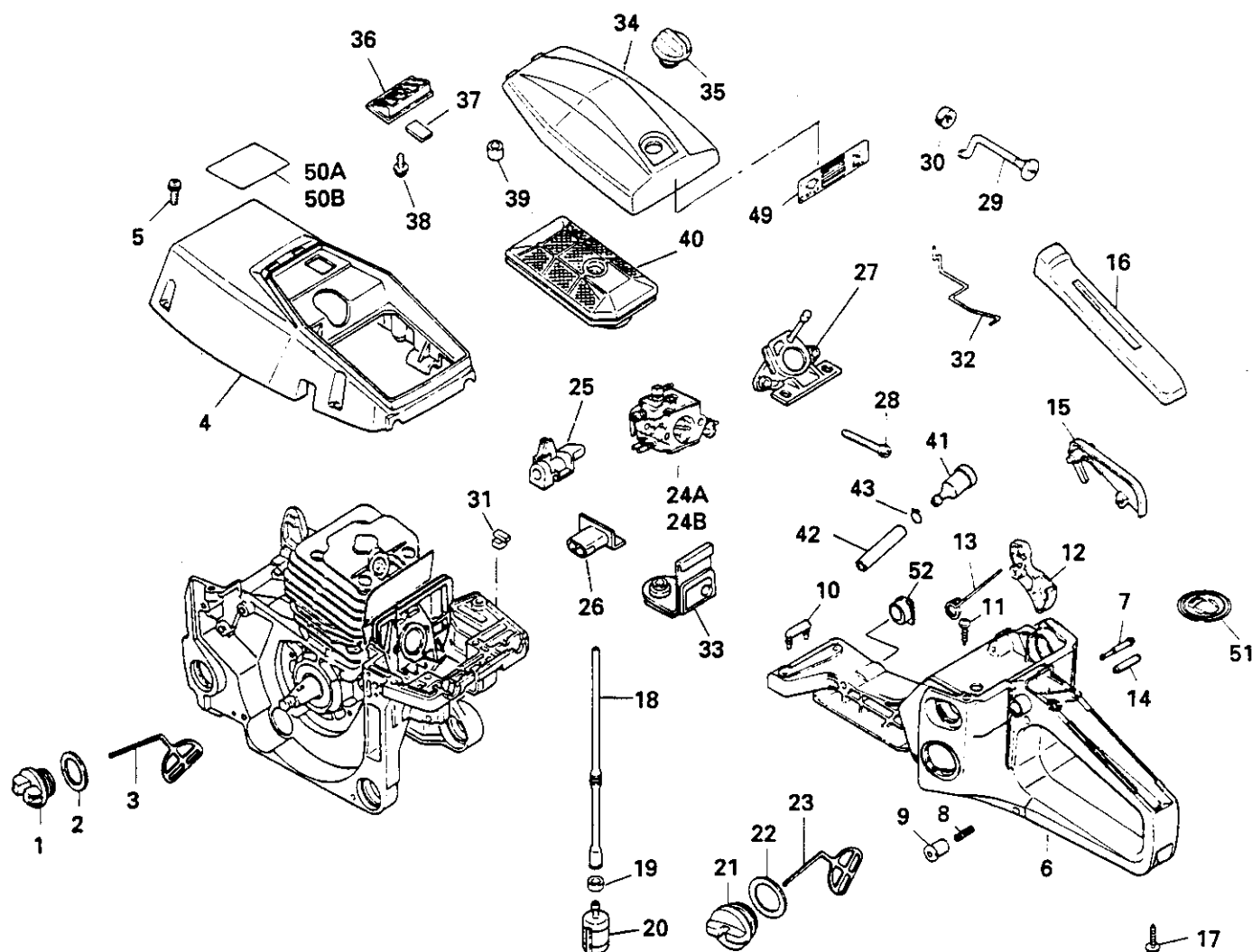
Fig. 3 REAR HANDLE, FUEL FEED LINE & AIR CLEANER
