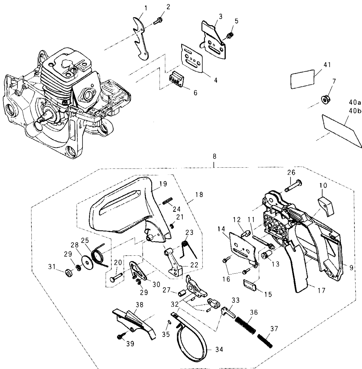
Fig. 6 BAR MOUNT, CHAIN BRAKE
