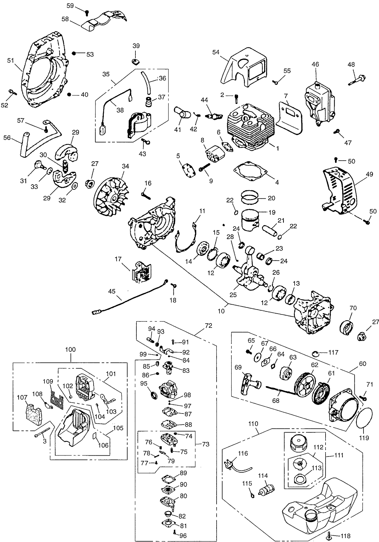
Fig.2 ENGINE GROUP
