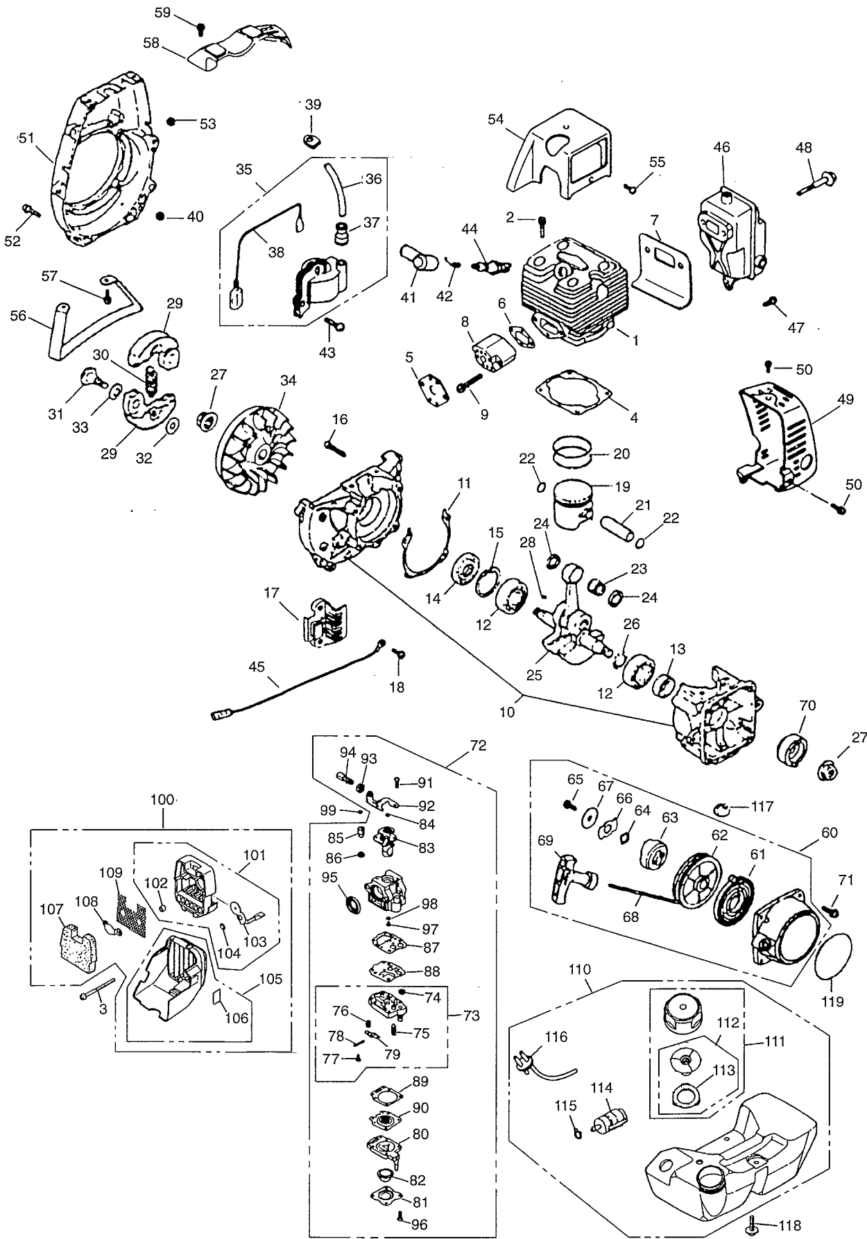
Fig.2 ENGINE GROUP
