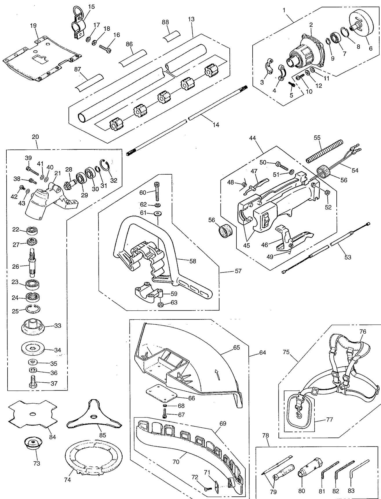
Fig.1 CUTTER GROUP
