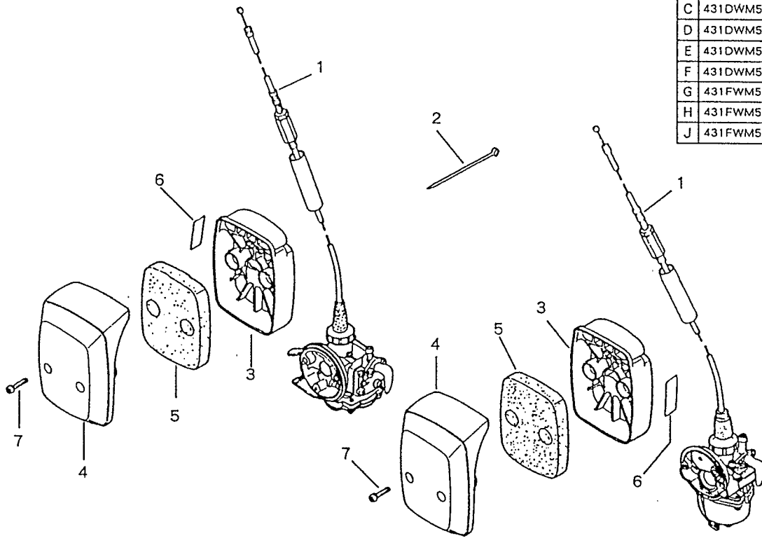
FIG. 6 THROTTLE CABLE &amp; AIR CLEANER
