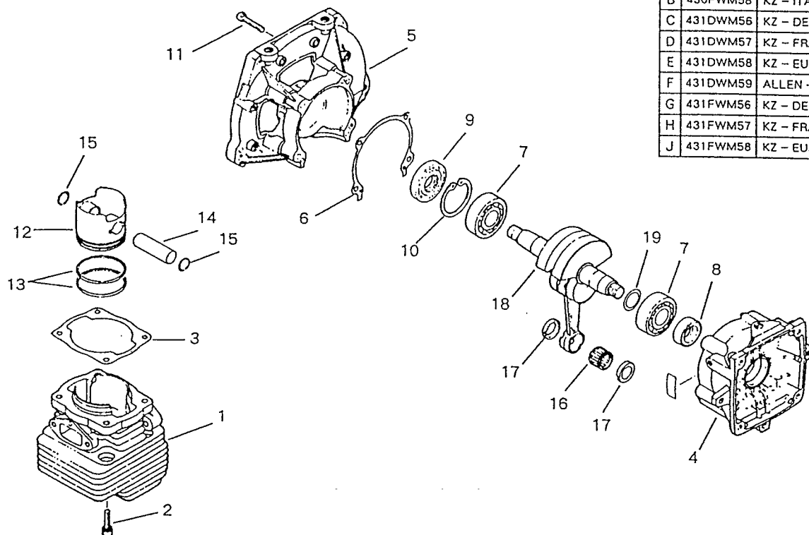
FIG. 1 ENGINE BLOCK
