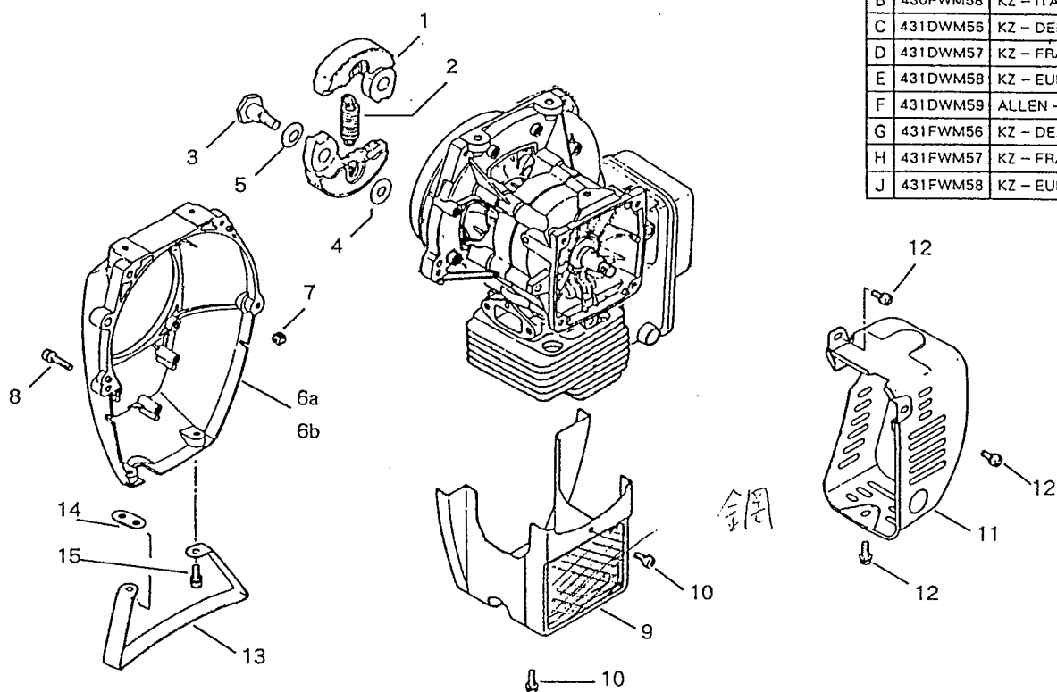
FIG. 5 CLUTCH &amp; COVERS
