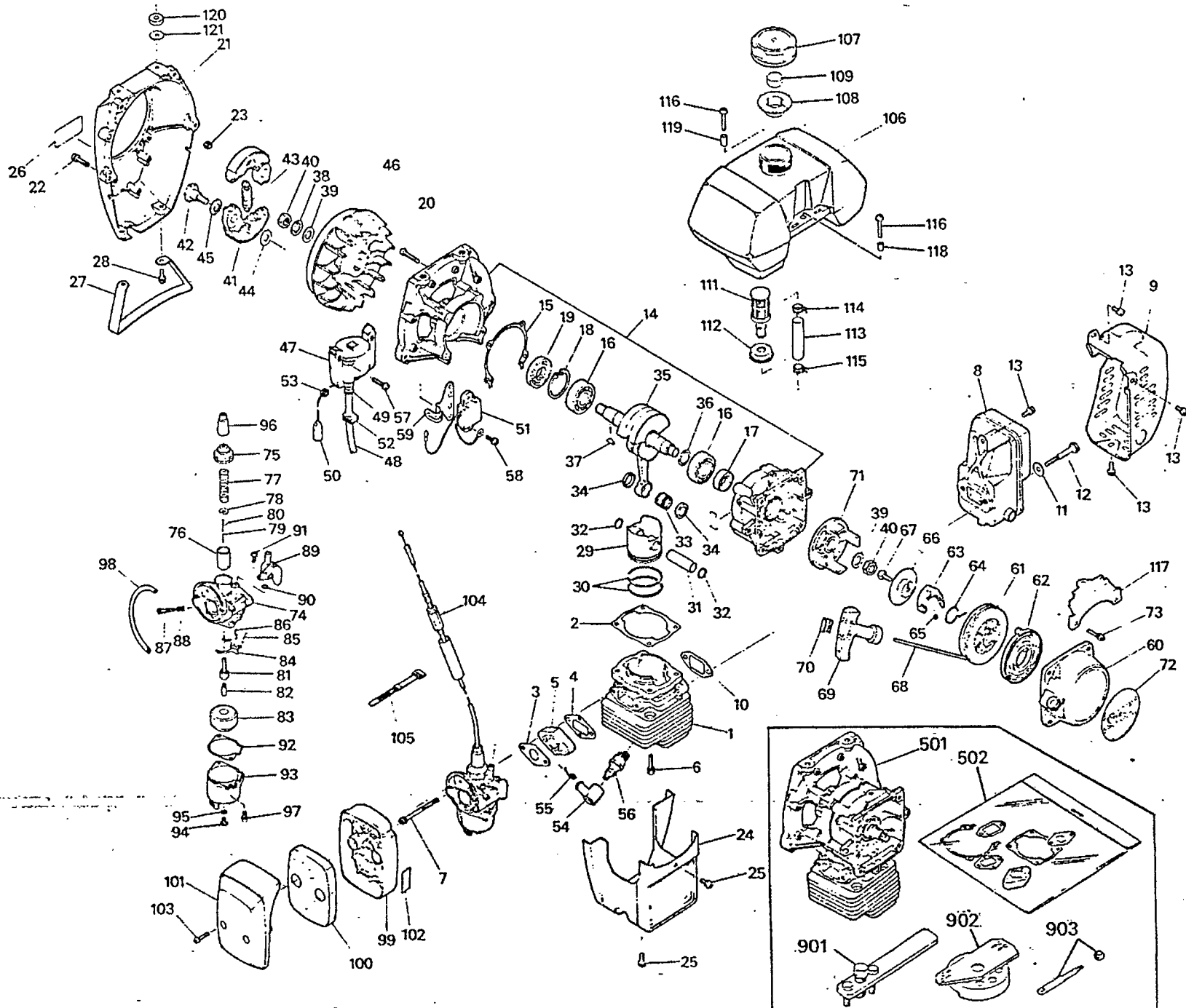
Fig. 1. ENGINE SECTION
