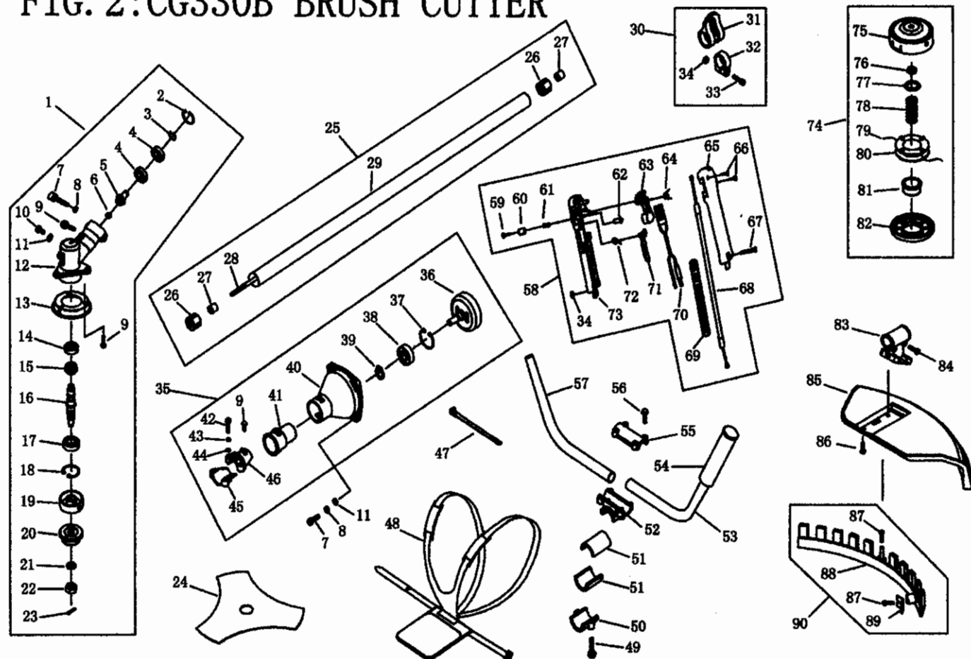
FIG. 2:CG330B BRUSH CUTTER
